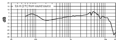
Typical Frequency Response
